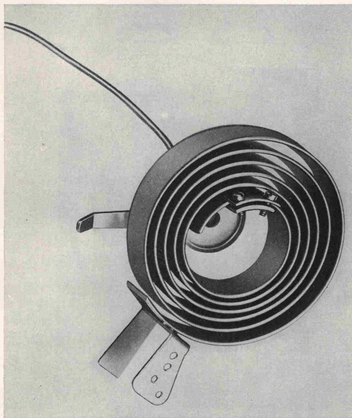
Fig. 4. Spiral pressure element.
